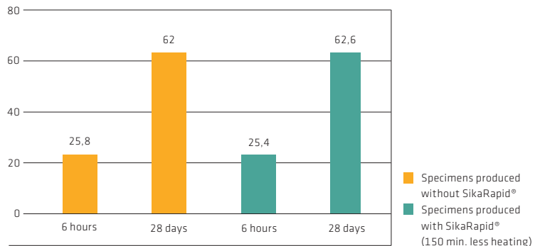
Concrete compressive strength [MPa]
