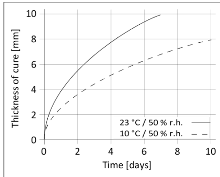
Diagram 1: Curing speed Sikaflex®-258 EP
