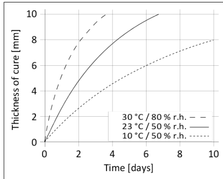
Diagram 1: Curing speed Sikaflex®-263
