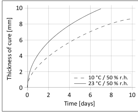
Diagram 1: Curing speed Sikaflex®-211 EMEA
